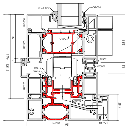
F82 CILL AND SUBCILL / D2
