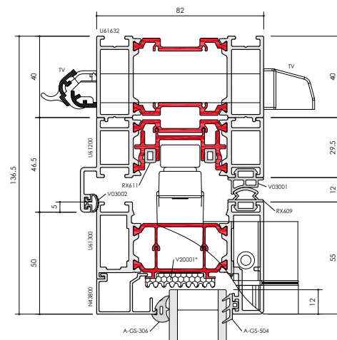
F82 HEAD WITH 40MM ADDON FOR TRICKLE VENT / A1
