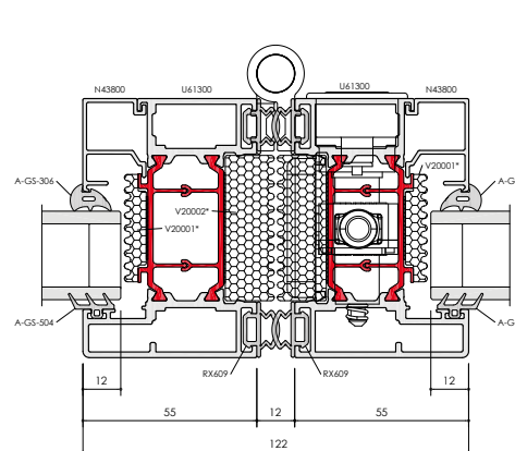
F82 MEETING STYLE / B
