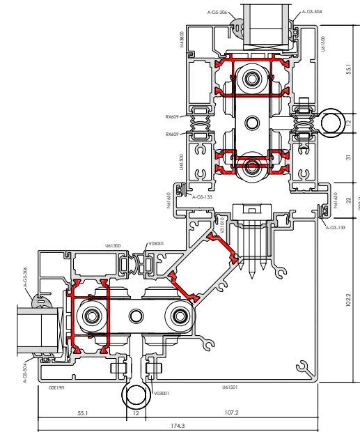
F82 FLOATING CORNER POST EVEN TO EVEN PANELS / C1
