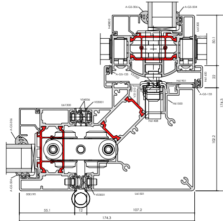
F82 FLOATING CORNER POST / C
