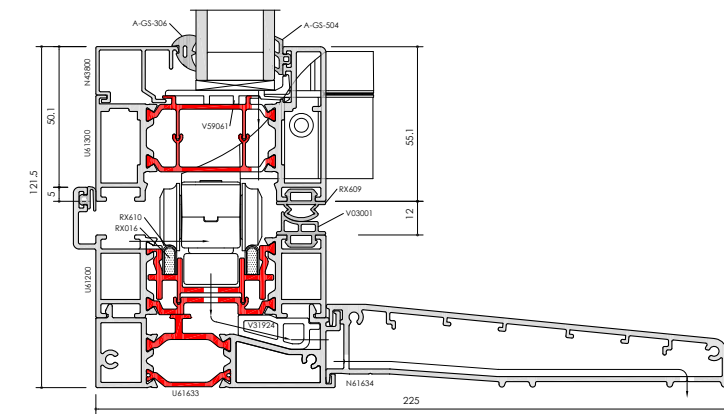
F82 CILL AND SUBCILL / D
