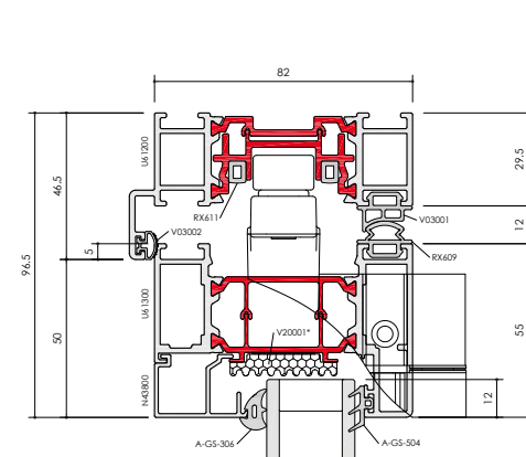
F82 HEAD / A
