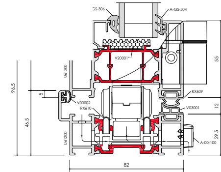
F82 WITH FACE DRAINAGE / D3
