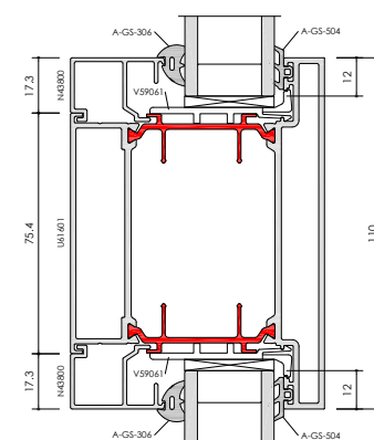
F82 MIDRAIL / E
