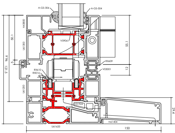
F82 CILL AND SUBCILL / D1
